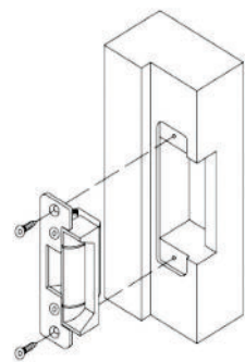
Mounting Installation on wooden door frame
