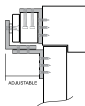
'L' & 'Z' BRACKET ARRANGEMENT
