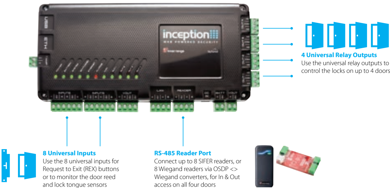
Four Door Access Control System
